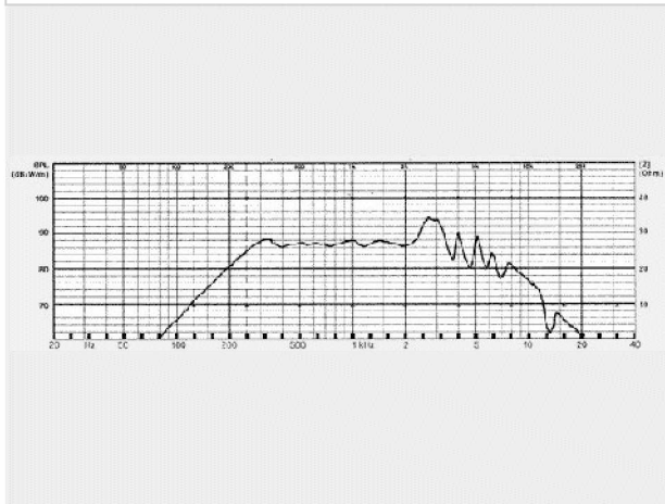
frequency response
