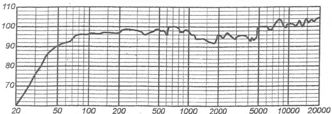
FREQUENCY RESPONSE CURVE
