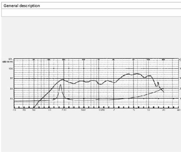
frequency response
