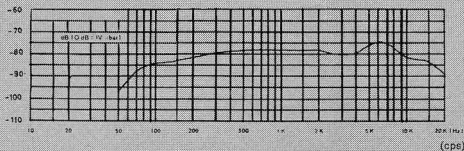
Nominal frequency response
