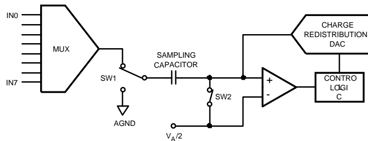
Figure 34. ADC128S052 in Track Mode
