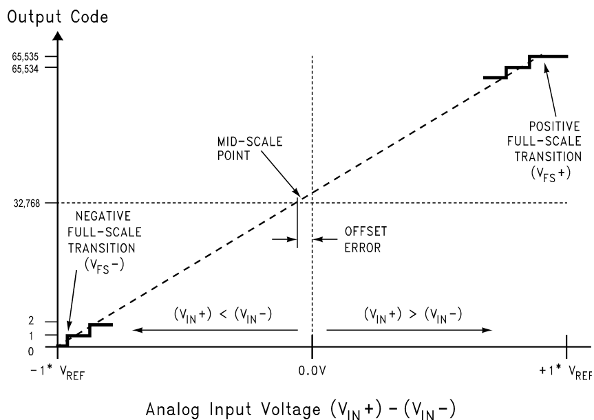
Figure 3. Transfer Characteristic (Offset Binary Format)
