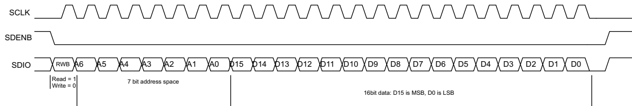
Figure 43. Serial Register Read Timing Diagram
