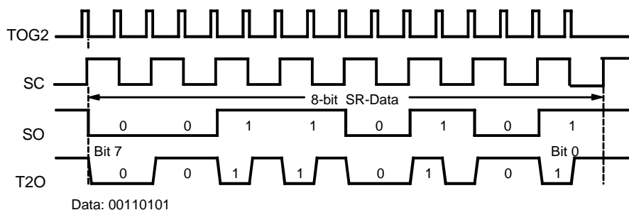
Figure 47. Biphase Modulation
