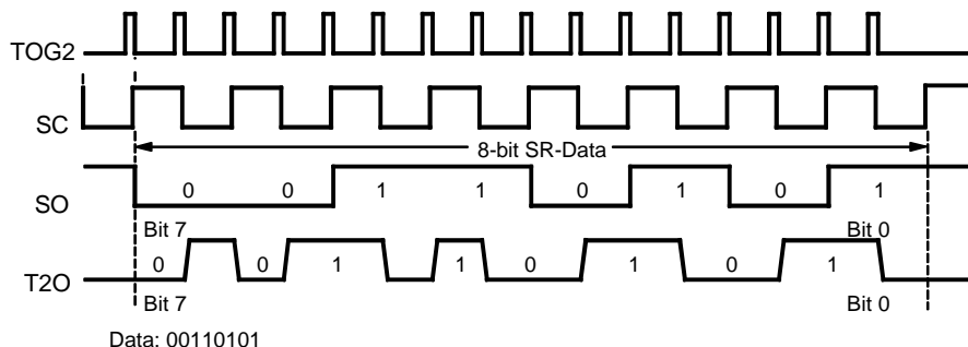
Figure 48. Manchester Modulation
