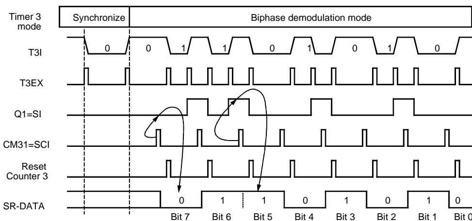
Figure 85. Biphase Demodulation
