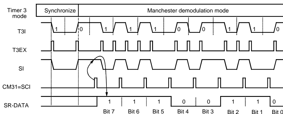
Figure 84. Manchester Demodulation
