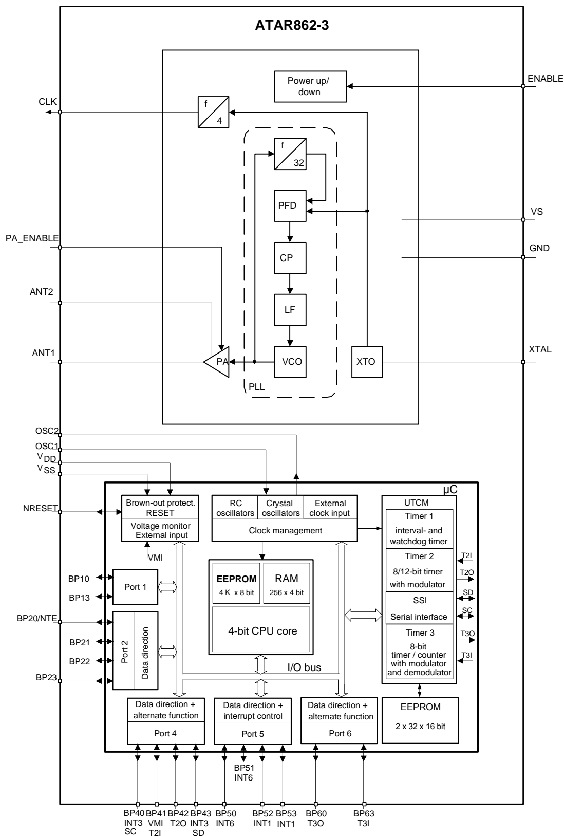
Figure 3. Block Diagram
