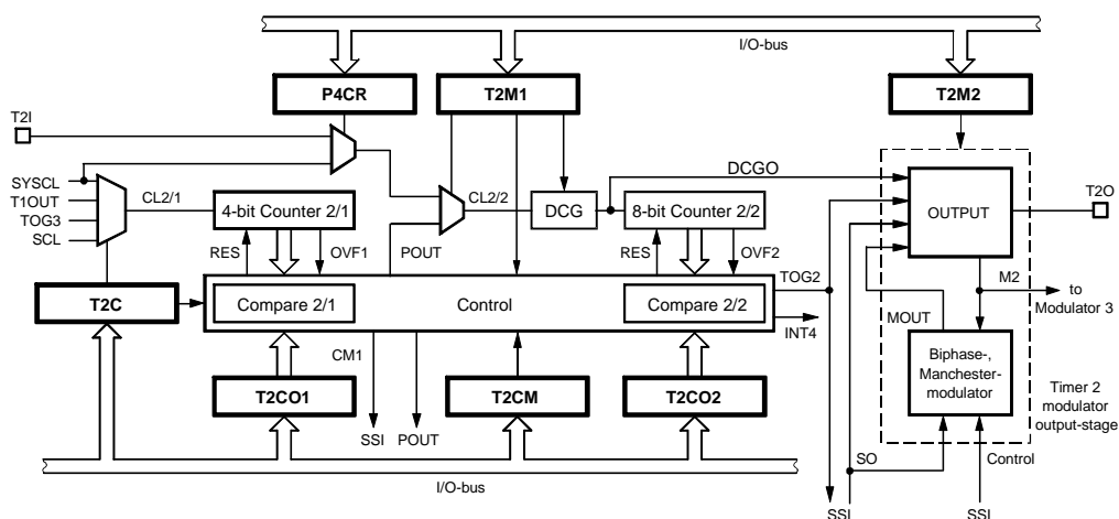
Figure 37. Timer 2
