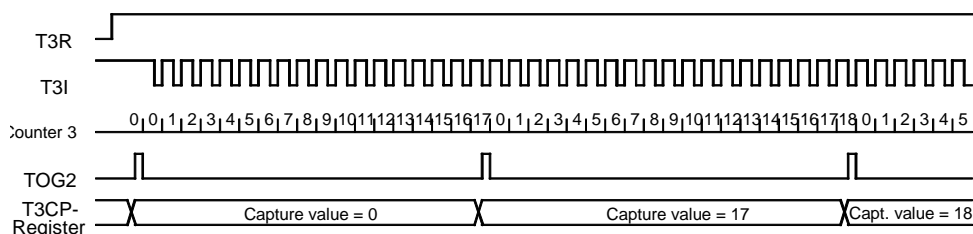
Figure 87. Frequency Measurement
