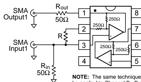
Figure 2: Optional Unity Gain Configuration
