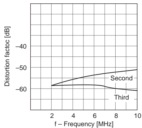
REC AMP distortion factor vs. Frequency
