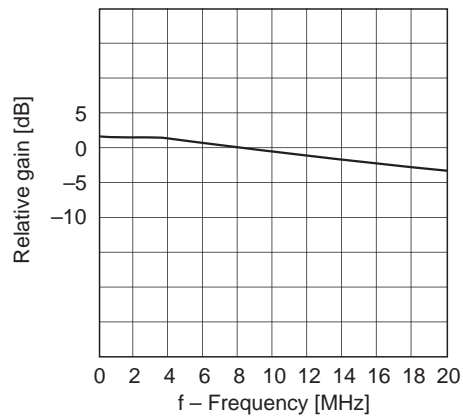
REC AMP frequency response
