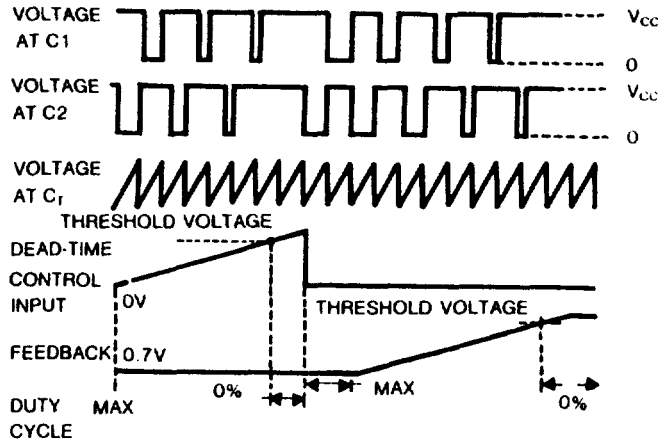
VOLTAGE WAVEFORMS
