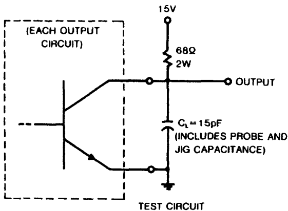
TEST CIRCUIT
