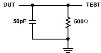
VOLTAGE LEVELS
