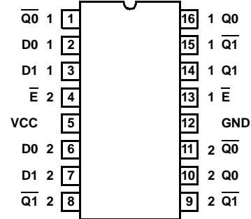
16 LEAD CERAMIC METAL SEAL FLATPACK PACKAGE (FLATPACK) MIL-STD-1835 CDFP4-F16, LEAD FINISH C TOP VIEW
