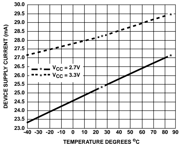
FIGURE 25. RECEIVE TOTAL SUPPLY CURRENT (LNA IN LOW GAIN)
