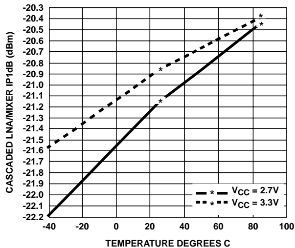
FIGURE 29. INPUT P1dB HIGH GAIN MODE
