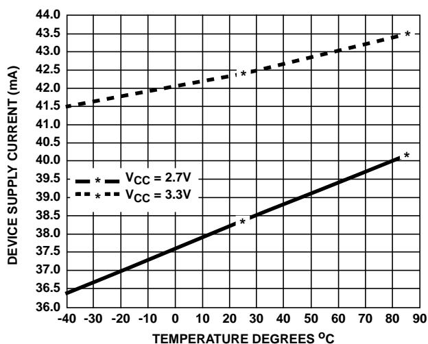
FIGURE 26. TRANSMIT TOTAL SUPPLY CURRENT
