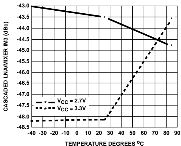
FIGURE 31. RX OUTPUT IM3 AT -5dBm INPUT TONES
