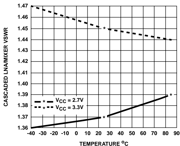
FIGURE 35. LNA INPUT 50Ω VSWR HIGH GAIN MODE
