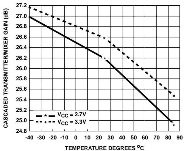
FIGURE 39. POWER CONVERSION GAIN
