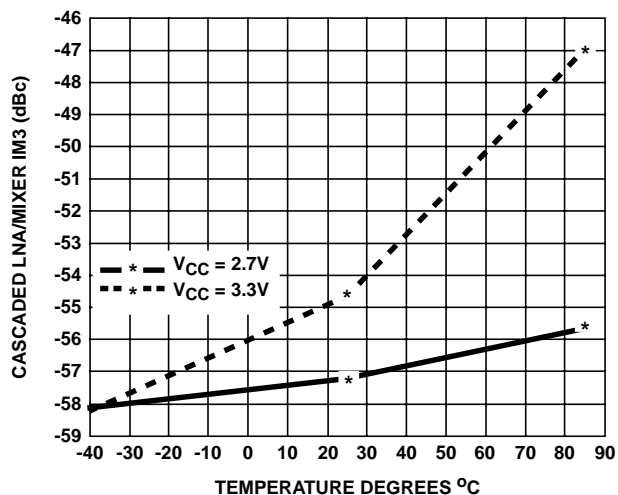
FIGURE 32. RX OUTPUT IM3 AT -12dBm INPUT TONES
