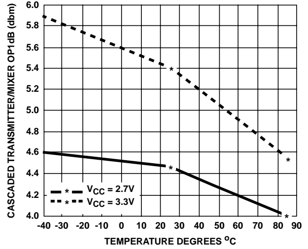
FIGURE 41. OUTPUT P1dB
