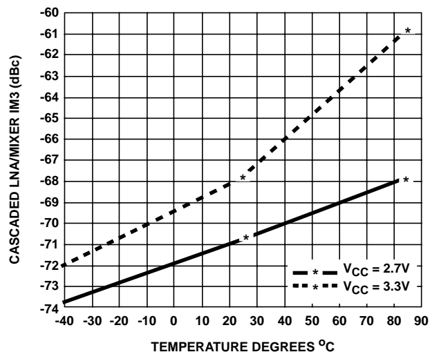
FIGURE 33. RX OUTPUT IM3 AT -20dBm INPUT TONES
