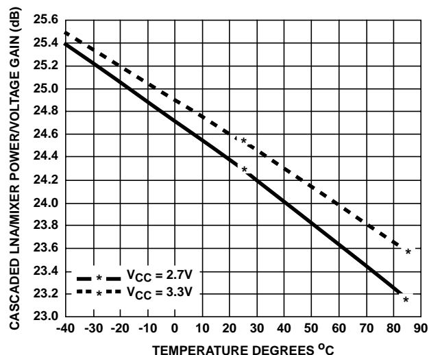
FIGURE 27. POWER/VOLTAGE GAIN HIGH GAIN MODE
