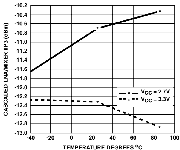
FIGURE 28. INPUT IP3 HIGH GAIN MODE
