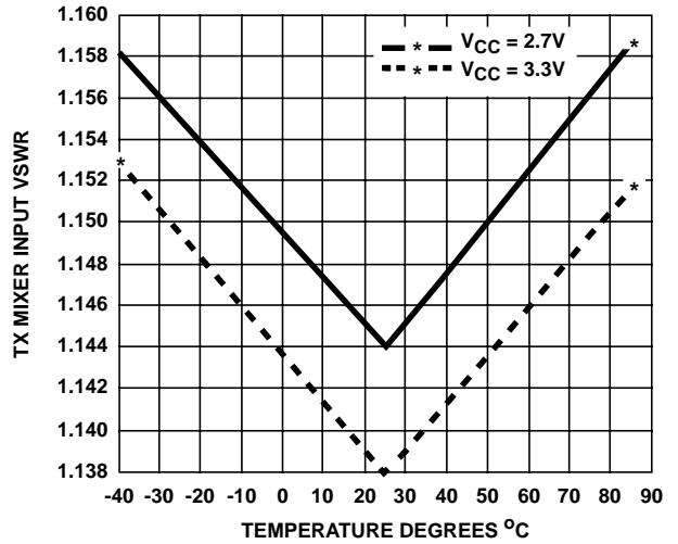
FIGURE 43. TX MIXER INPUT VSWR
