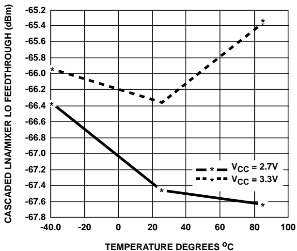
FIGURE 38. LO TO LNA INPUT FEEDTHROUGH (CASCADED, NO FILTER)
