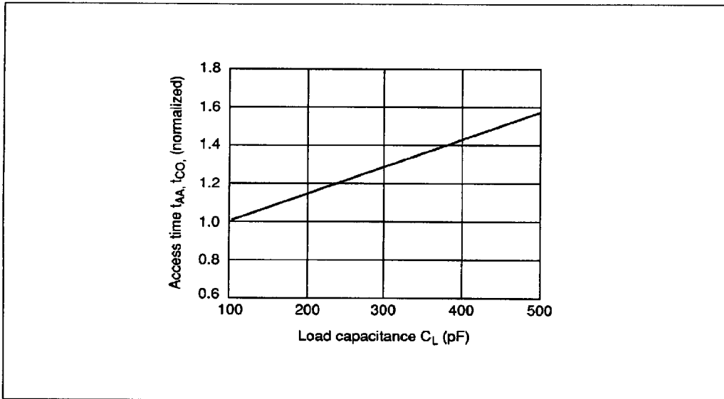
Access Time vs. Load Capacitance
