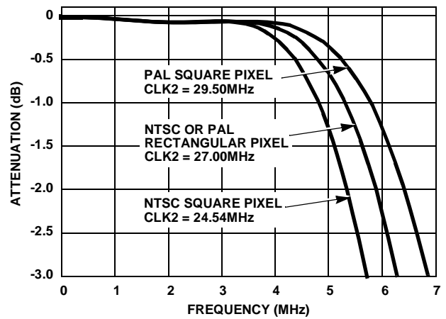
FIGURE 7B. PASS BAND
