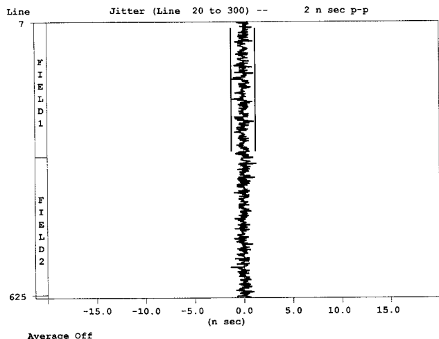
FIGURE 24. H SYNC JITTER IN A FRAME (PAL)
