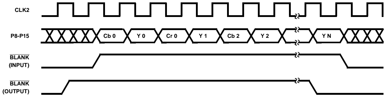
FIGURE 1. PIXEL INPUT TIMING - 8-BIT YCBCR
