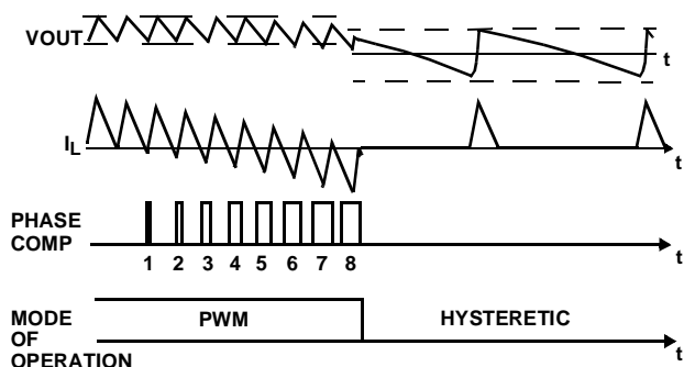
FIGURE 2. HYSTERETIC OPERATION MODE
