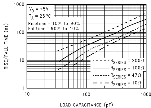
\phi 1, \phi 2, RS , and TR Rise and Fall Times Through A Series Resistance vs Load Capacitance
