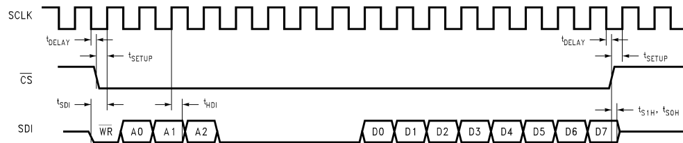
FIGURE 13. Configuration Register Write Timing using \overline{CS} , Continuous SCLK (16-Bit Word)
