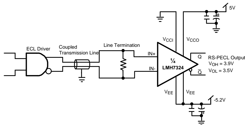
Figure 6. ECL TO RSPECL
