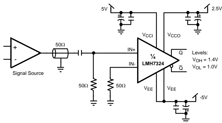
Figure 8. ANALOG TO LVDS
