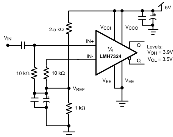
Figure 9. Standard Setup
