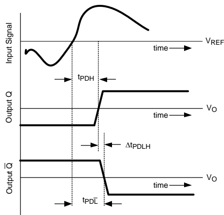
Figure 11. t_{PD} with Complementary Outputs
