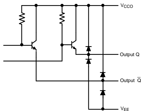
Figure 3. Equivalent Output Circuitry
