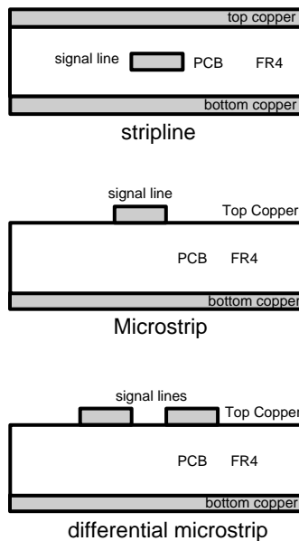
Figure 22. PCB Lines
