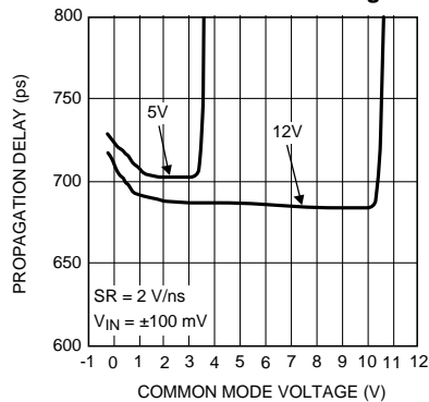
Propagation Delay vs. Common Mode Voltage
