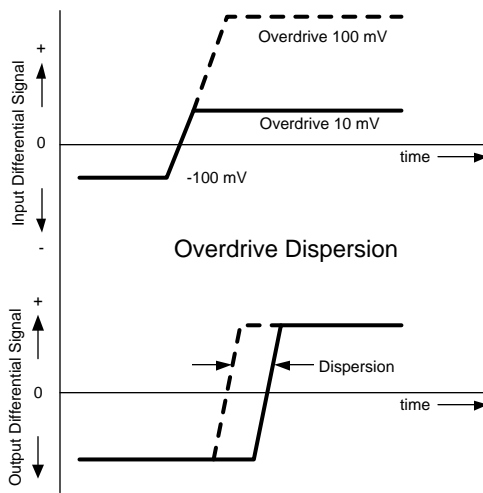
Figure 12. Overdrive Dispersion
