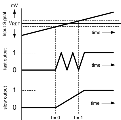
Figure 15. Oscillations on Output Signal
