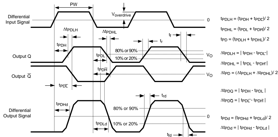
Figure 4. Timing Definitions
