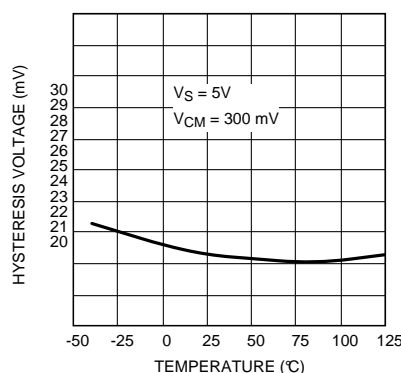
Figure 17. Hysteresis Voltage over Temperature
