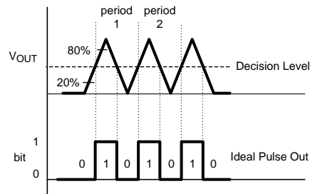
Figure 20. Bit Rates
