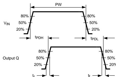
Figure 10. Propagation Delay
