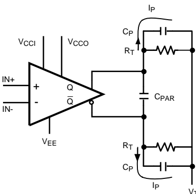
Figure 19. Parasitic Capacities
