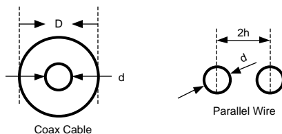
Figure 21. Cable Types
