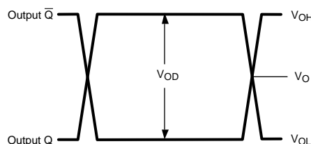
Figure 18. Output Swing
