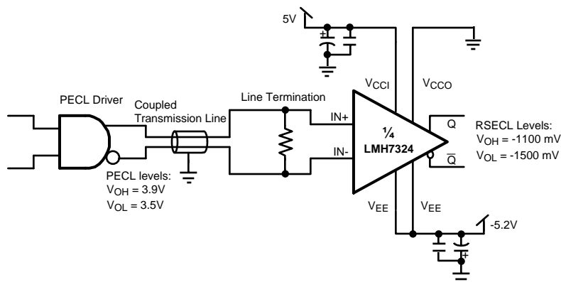
Figure 7. PECL TO RSECL
