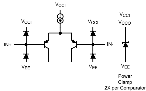
Figure 2. Equivalent Input Circuitry
