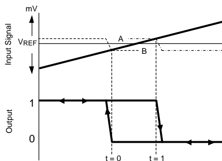
Figure 16. Hysteresis
