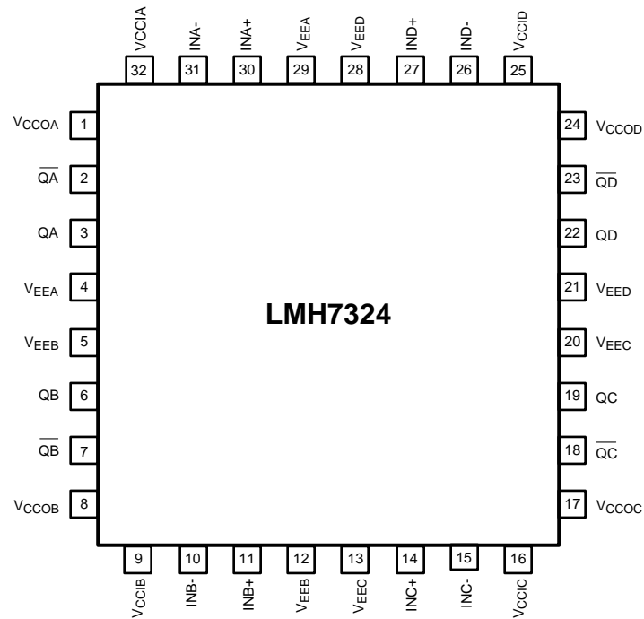
Figure 1. Top View
