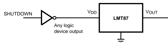
Figure 13. Conserving Power Dissipation with Shutdown
