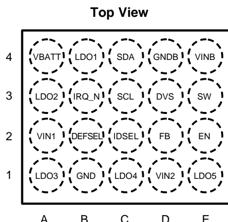
Figure 1. DSBGA Package See Package Number YZR002011A
