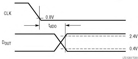
Voltage Waveform for D_{OUT} Delay Time, t_{dO}
