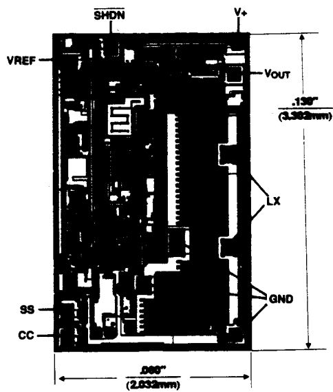
Chip Topography
