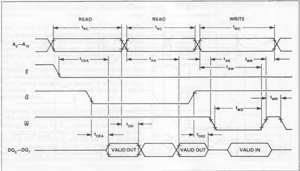
FIGURE 3. READ-READ-WRITE TIMING
