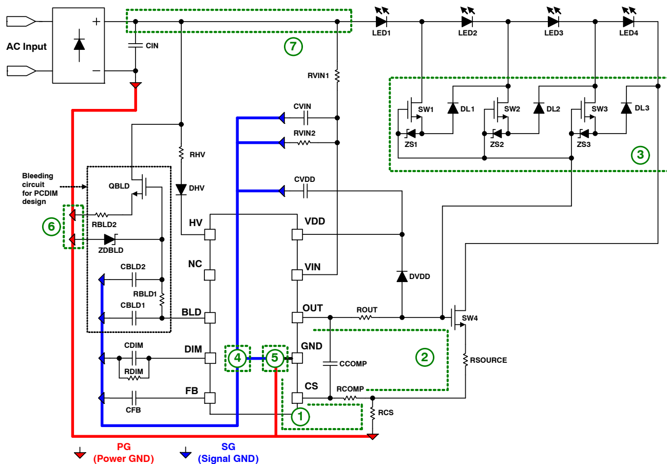
Figure 15. System Layout
