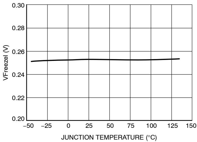
Figure 13. VFreezeI vs. Junction Temperature
