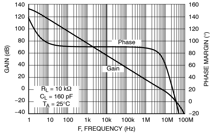
Figure 12. Error Amplifier Open Loop Response
