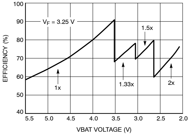
Figure 4. Efficiency vs. V_{\text{BAT}} Voltage
