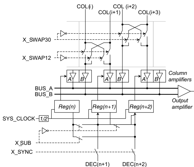
Figure 9. Column Structure
