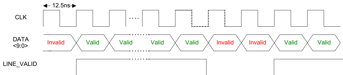
Figure 20. LINE_VALID Timing
