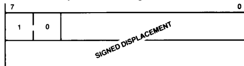
Word Displacement: Range -8192 to +8191
