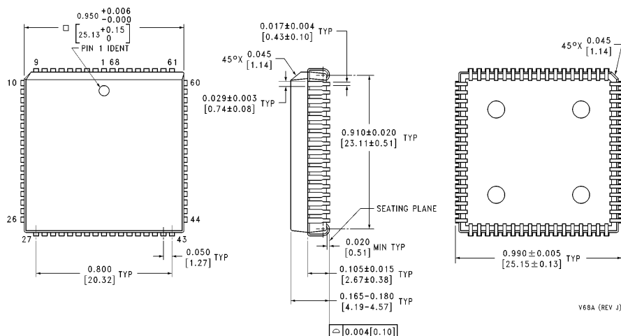
68-Pin Plastic Leaded Chip Carrier (V) Order Number NSAM266SCA/V NS Package Number V68A
