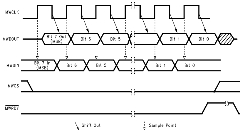
FIGURE 2-3. Sequence of Activities during a MICROWIRE Byte Transfer
