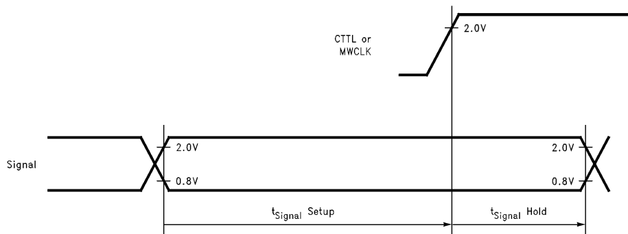
FIGURE 1-12. Synchronous Input Signals
