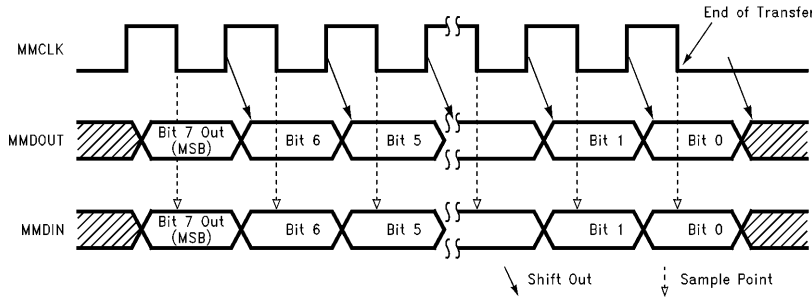
FIGURE 2-4. Master MICROWIRE Data Transfer
