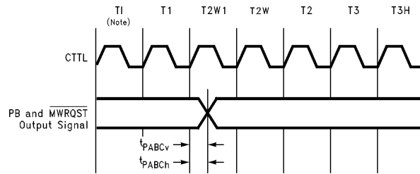
FIGURE 1-21. Output Signal Timing for Port PB and MWRQST
