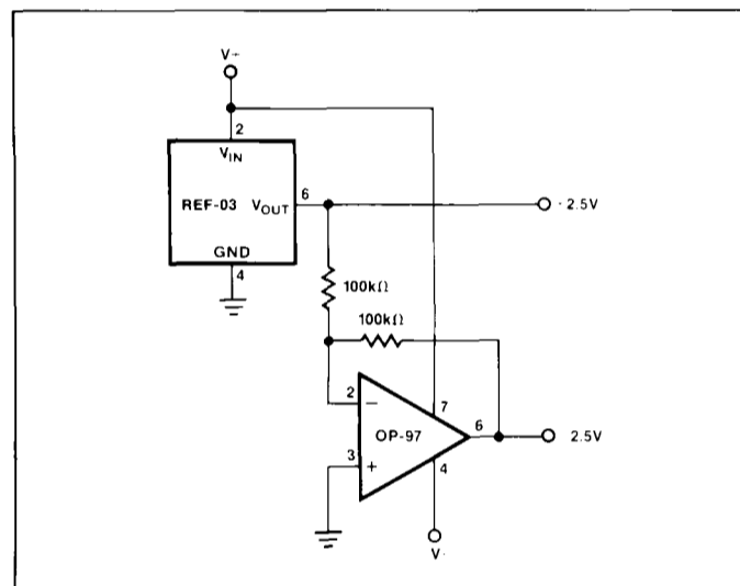
FIGURE 3: ±2.5V Reference
