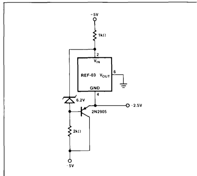
FIGURE 4: -2.5V Reference
