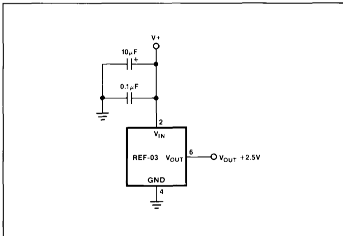
FIGURE 1: Basic Connections
