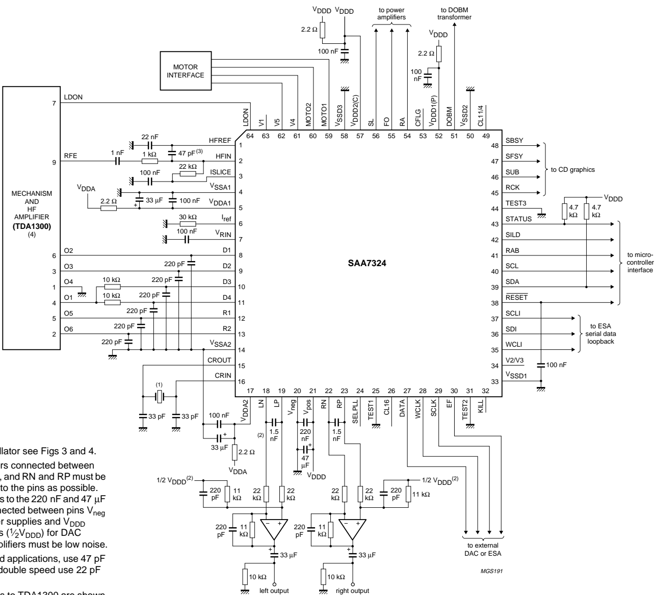
Fig.38 Typical application diagram (for current mechanisms).
