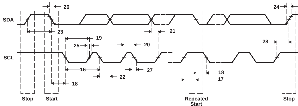
Figure 5-37. I²C Transmit Timings
