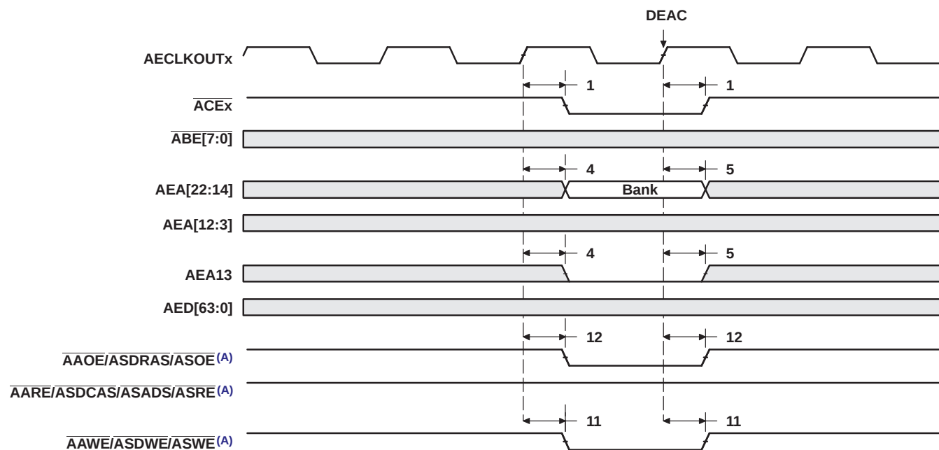
Figure 5-26. SDRAM DEAC Command for EMIFA
