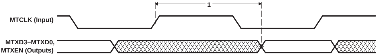
Figure 5-66. EMAC Transmit Interface Timing
