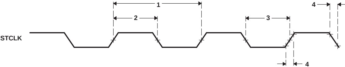
Figure 5-62. STCLK Timing
