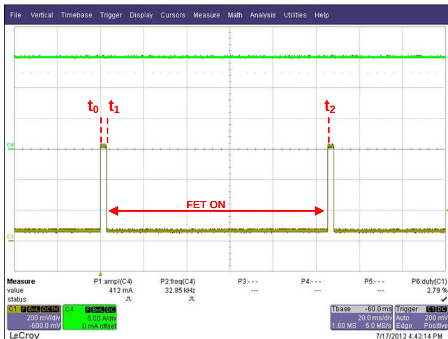
Figure 6. ANODE to CATHODE voltage (Ch1) with I_{\text{BYPASS}} = 15\text{A} (Ch4) for SM74611 in Junction Box at 85^\circ\text{C} ambient
