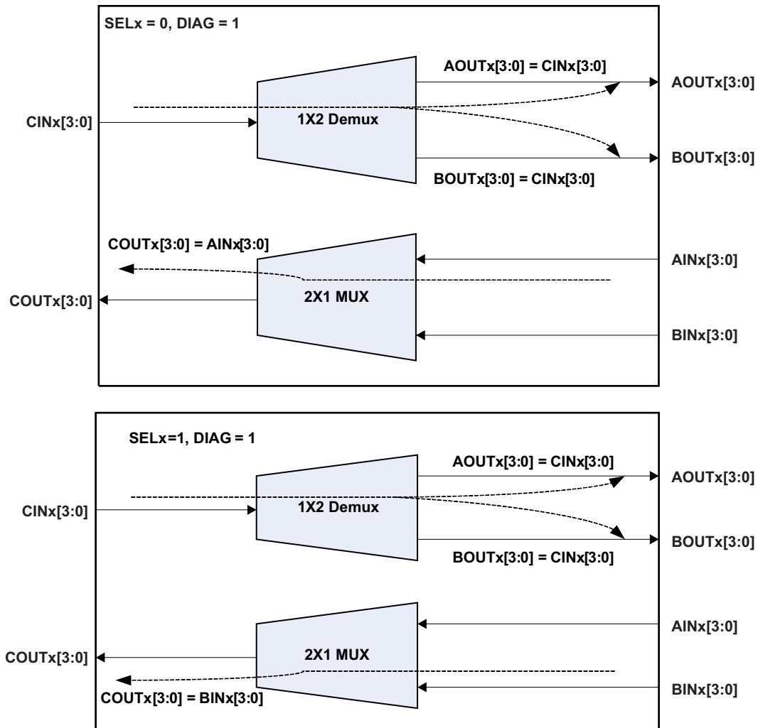
Figure 14. Diagnostic Mode
