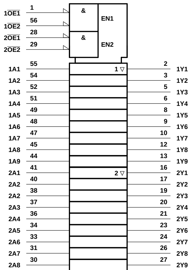
LOGIC SYMBOL (1)
