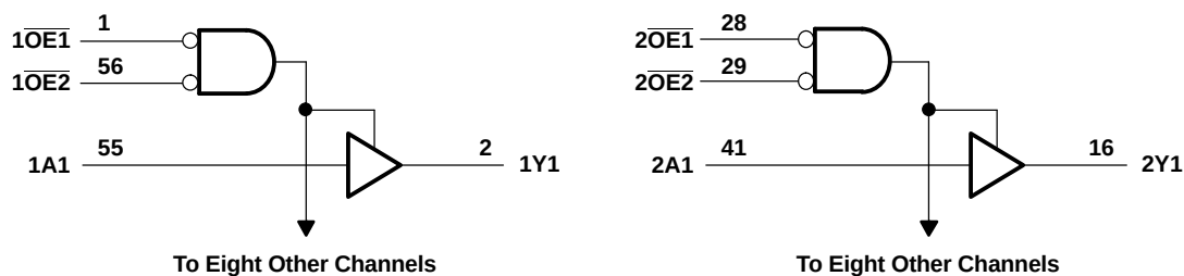
LOGIC DIAGRAM (POSITIVE LOGIC)
