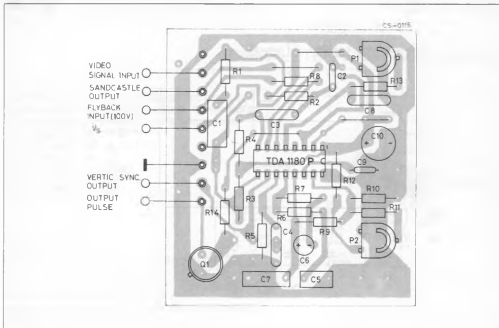
Figure 8 : Application Circuit for Small Screen b.w. TV.
