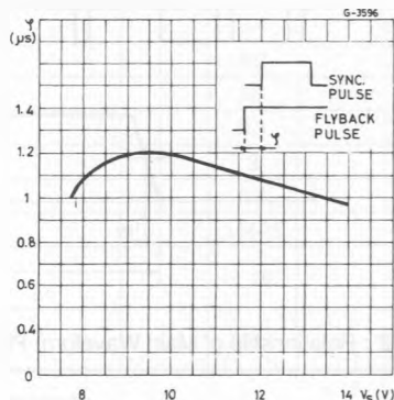
Figure 4 : Overall Phase Relation vs. Supply Voltage.
