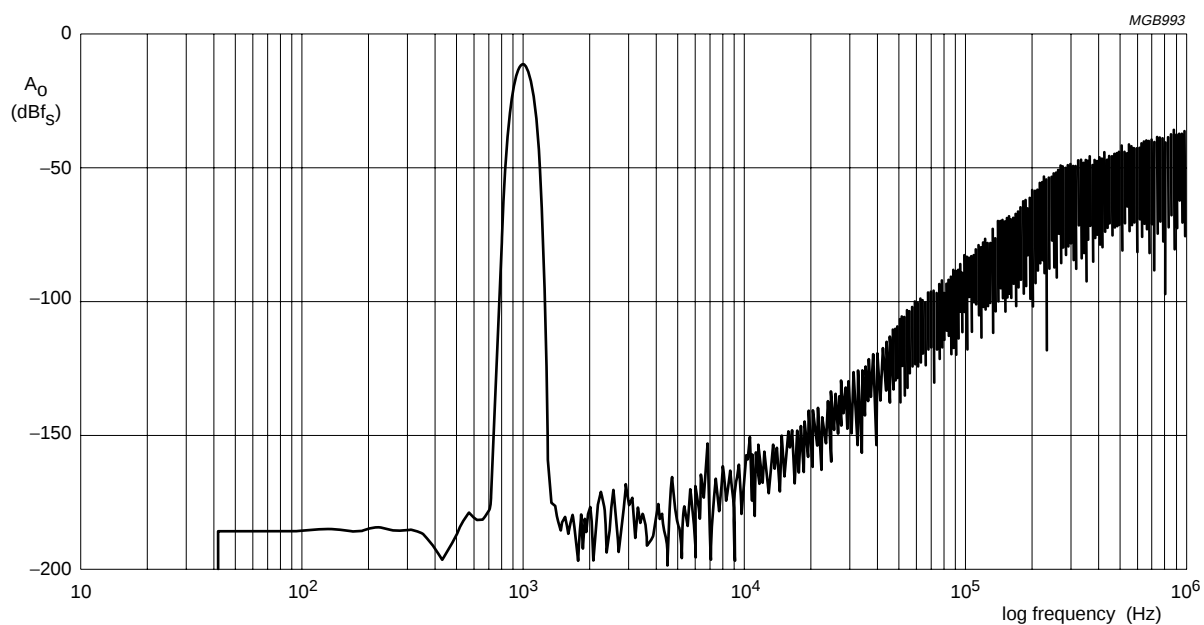
Fig.16 Noise shaper output spectrum ( N = 4 ; 192f_s ).
