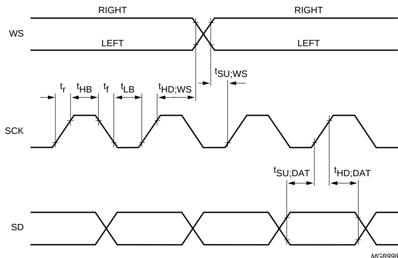
Fig.10 Typical I 2 S-bus data waveforms.
