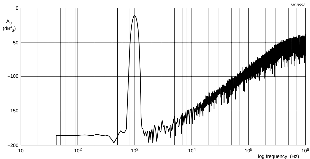
Fig.15 Noise shaper output spectrum ( N = 3 ; 192f_s ).
