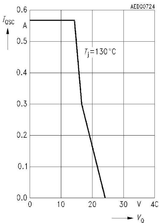
Short-Circuit Current I_{Q0} versus Output Voltage V_Q (0.5 A outputs)
