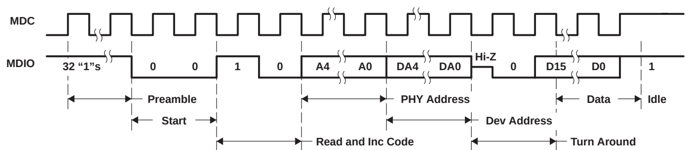
Figure 3-24. Management Interface Extended Space Read and Increment Timing
