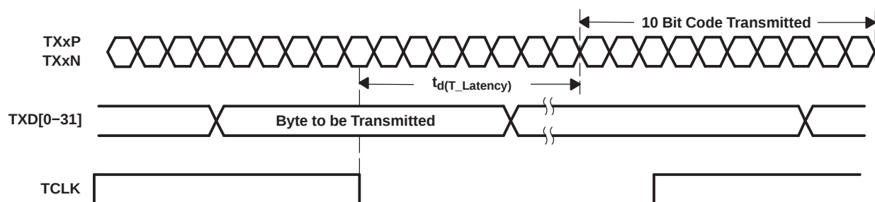
Figure 8. Transmission Latency
