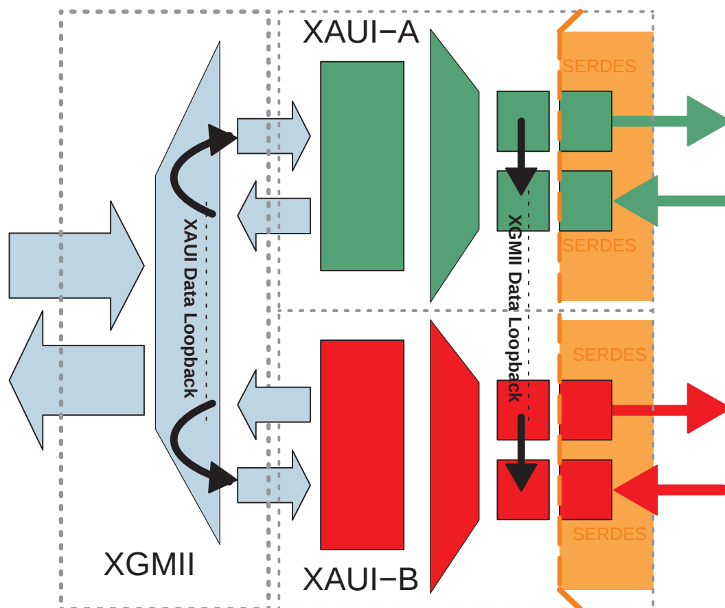
Figure 20. Data Loopback
