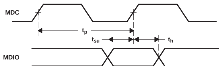
Figure 35. MDIO Read/Write Timing Diagram
