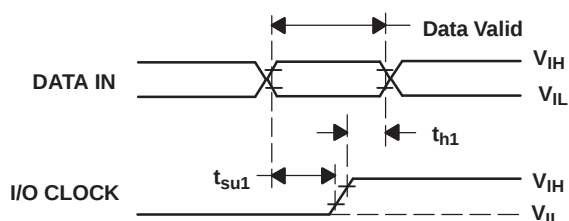
Figure 38. DATA IN and I/O CLOCK Voltage Waveforms
