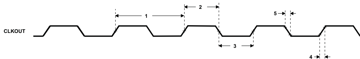
Figure 6-10. CLKOUT Timing
