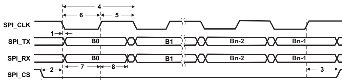
Figure 6-32. SPI Mode 2 Transfer (CKPn = 1, CKPHn = 0)
