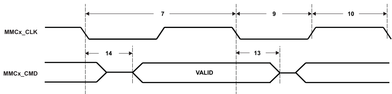
Figure 6-21. MMC/SD Host Command Write Timing
