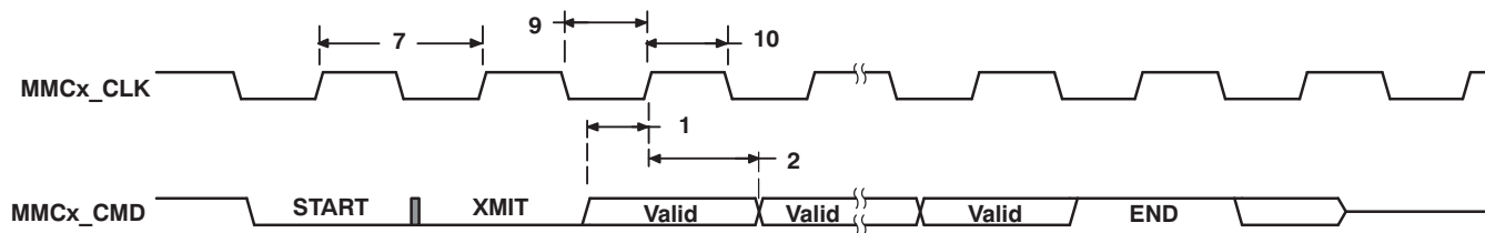
Figure 6-23. MMC/SD Host Write Timing
