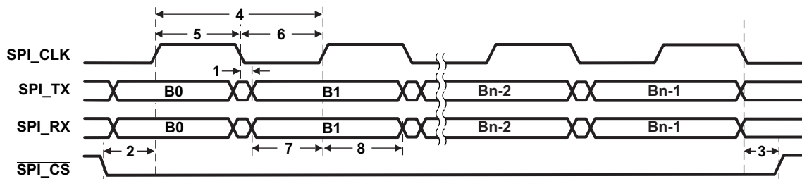
Figure 6-30. SPI Mode 0 Transfer (CKP n = 0, CKPH n = 0)
