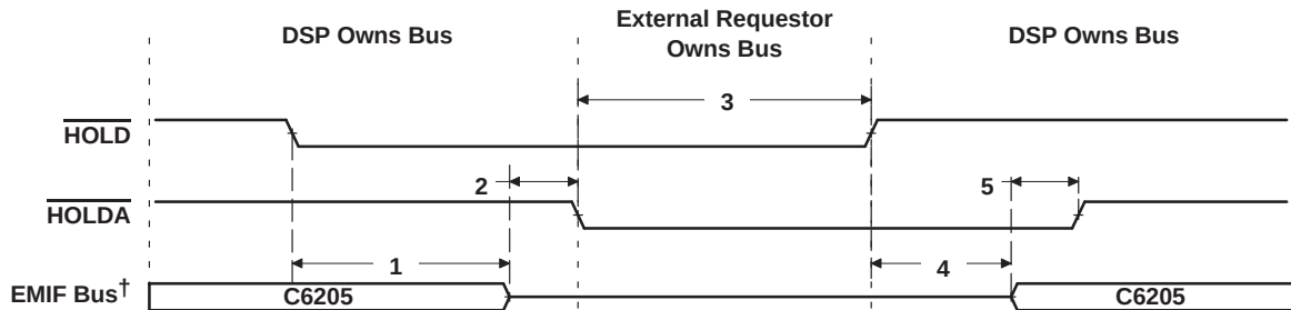
Figure 27. \overline{\text{HOLD}}/\overline{\text{HOLDA}} Timing
