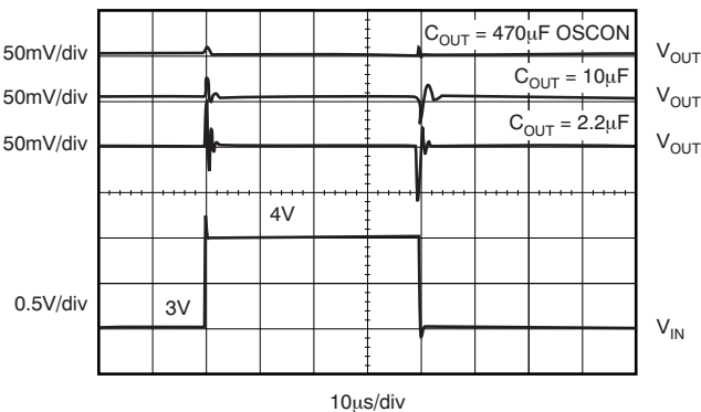
TPS73525 LINE TRANSIENT RESPONSE
