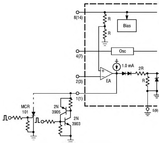
Figure 31. Latched Shutdown
