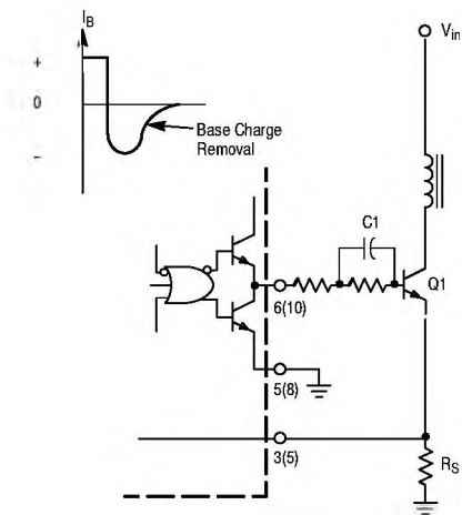
Figure 29. Bipolar Transistor Drive
