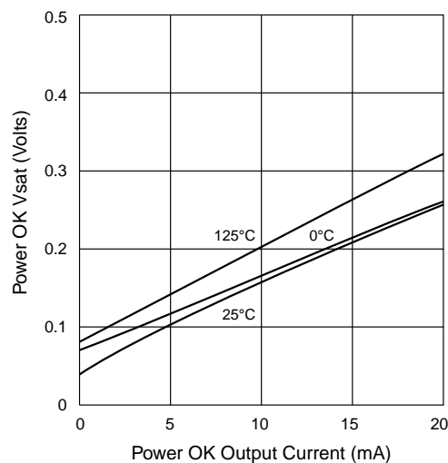
PWROK Saturation Voltage
