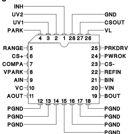
PLCC-28 (Top View) QP Package
