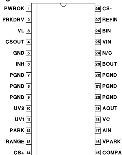
SOIC-28 (Top View) DWP Package
