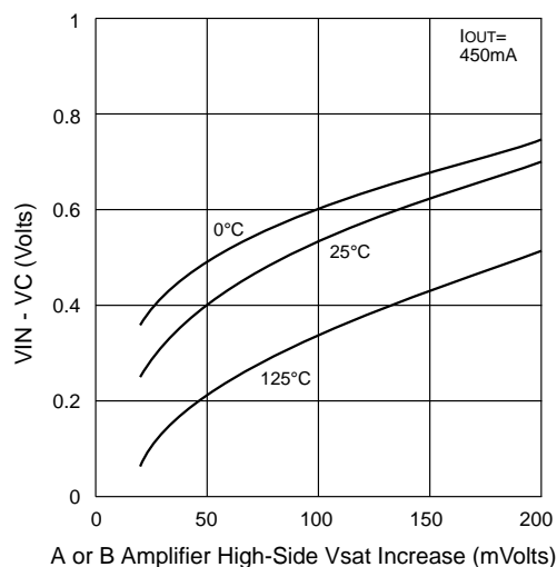
VIN to VC Headroom
