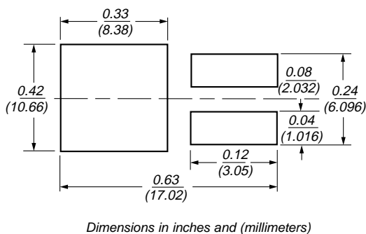
Mounting Pad Layout TO-263AB
