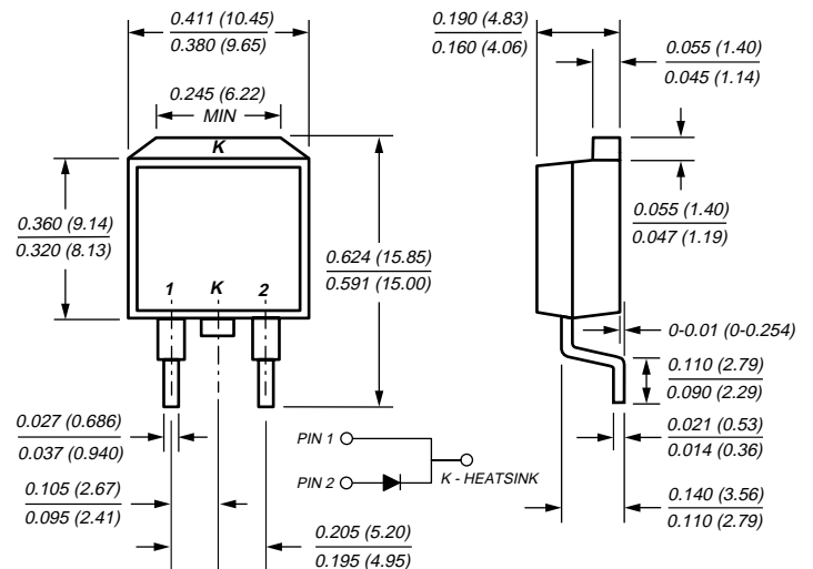
TO-263AB (BYWB29 Series)
