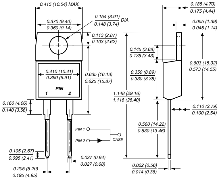
TO-220AC (BYW29 Series)
